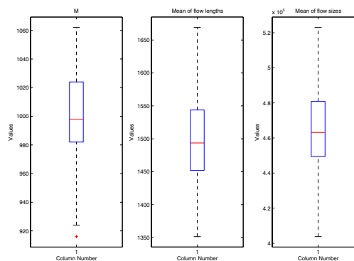
Fig. 7. Boxplots for various parameters of a mixture distribution
