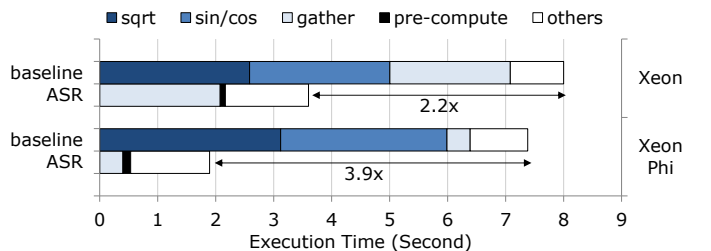
Fig. 7: Performance improvements of backprojection from ASR. Images with 3K \times 3K size are reconstructed from 2,809 pulses with 4K samples each.
