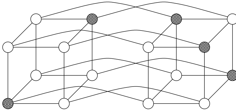
5 faulty nodes destroying every 2-cube
