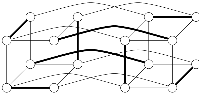
8 faulty edges destroying every 2-cube
