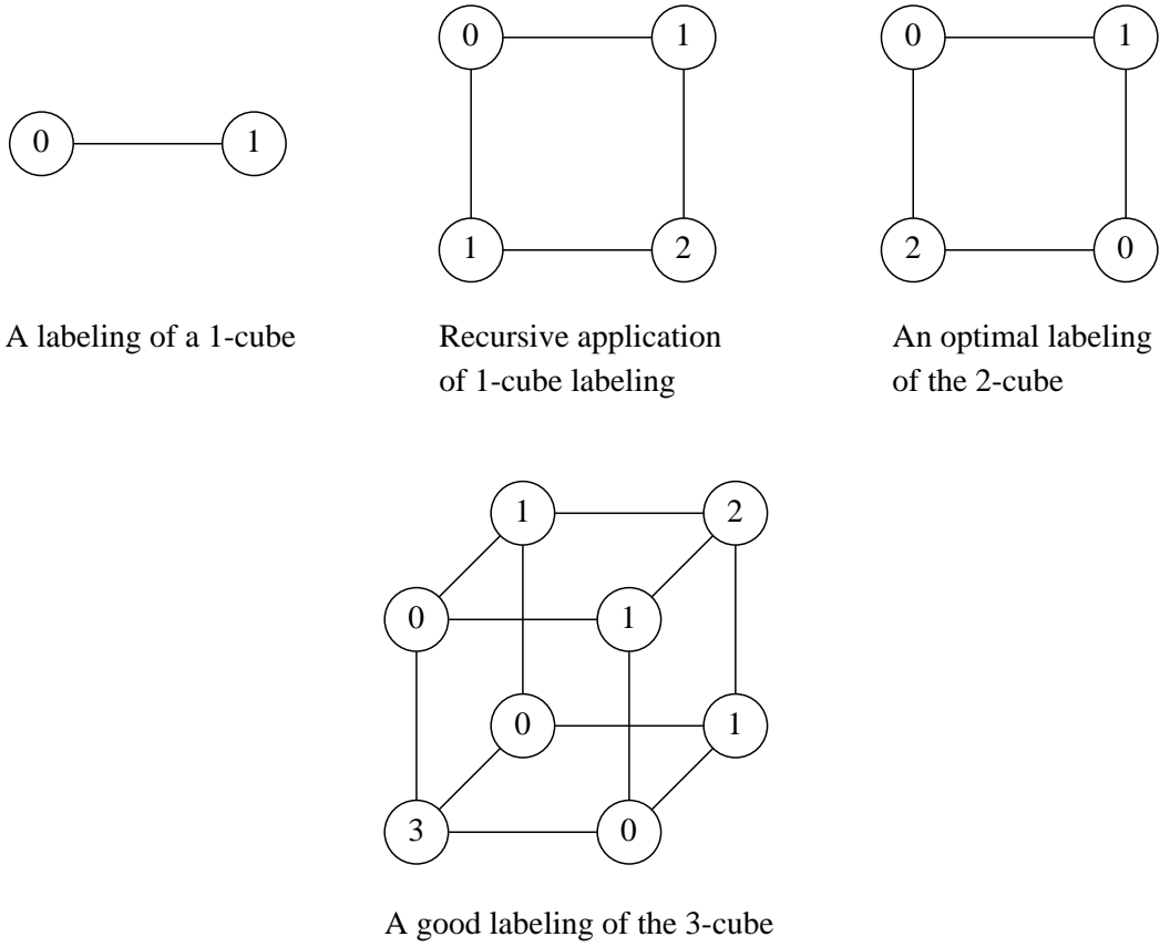
Figure 2: Labelings of small hypercubes
