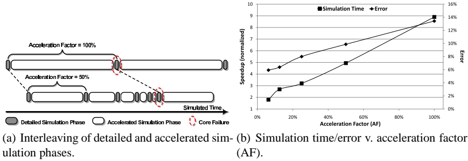
Fig. 5. The adaptive simulation used to accelerate lifetime reliability simulations while incurring minimal experimental error.
