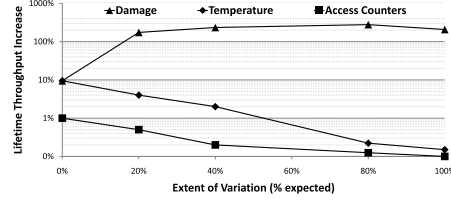
Fig. 9. Performance of wearout-centric scheduling with different sensors.
