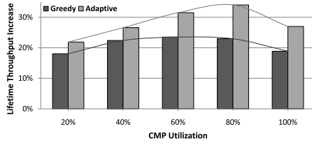
Fig. 8. Impact of CMP utilization on reliability enhancement.
