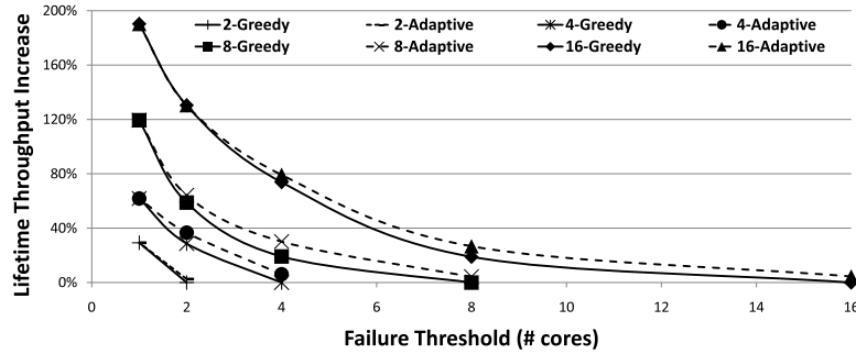
Fig. 6. Performance of wearout-centric scheduling policies verses CMP size and failure threshold.
