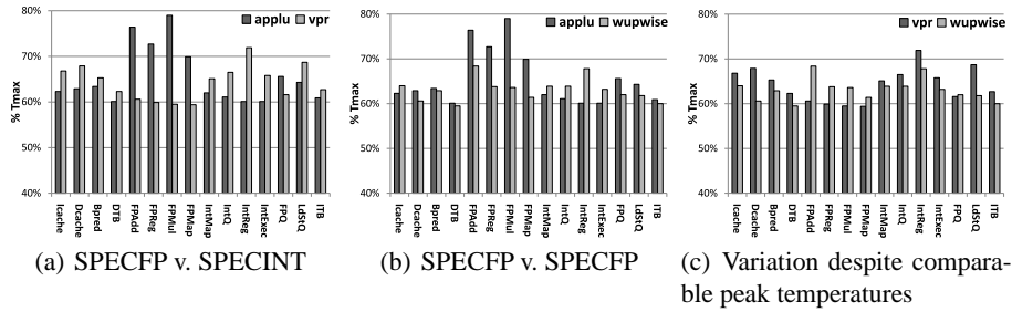
Fig. 2. Head-to-head comparisons of applu (SPEC FP), vpr (SPEC INT), and wupwise (SPEC FP). No one benchmark in (a), (b), or (c) strictly dominates the other (with respect to temperature) across all modules.
