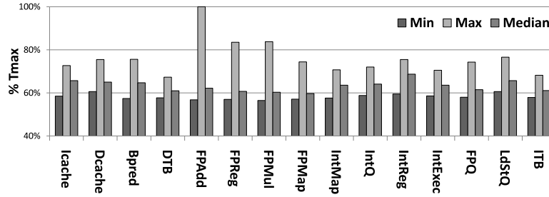
Fig. 1. Variation of module temperatures across SPEC2000 workloads. All temperatures are normalized to T_{max} , the peak temperature seen across all benchmarks and modules ( 83^{\circ}\text{C} ).
