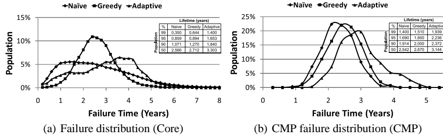
Fig. 7. Failure distributions for individual cores and the 16-core CMP with a failure threshold of 8 cores and 100% utilization. Trendlines are added (between markers) to improve readability.
