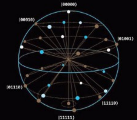
QSPHERE (5 QUBITS)
