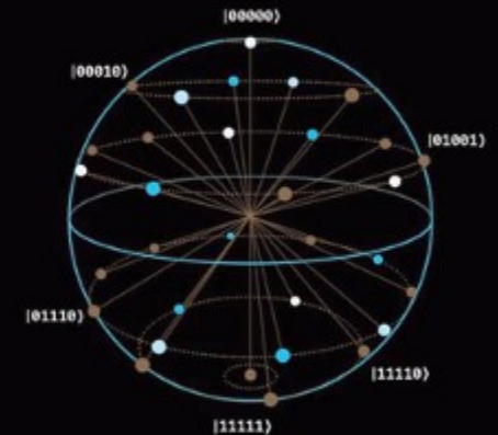
QSPHERE (5 QUBITS)
