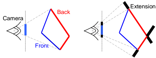
Figure 4: Silhouettes. Back-facing polygons in red before (left) and after enlargement (right).
