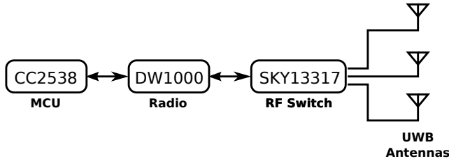
(a) Node Architecture
