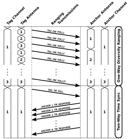
Figure 4: Ranging protocol. PolyPoint is able to leverage antenna diversity without significantly impacting position update rate. The protocol starts with a series of 27 broadcast transmissions from the tag for each combination of tag antenna, anchor antenna, and RF channel. The time-of-arrival data collected from this sequence provides information on the difference between all range estimates throughout the sequence. Finally, a two-way time-of-flight handshake is sent to determine the true range estimate for the first configuration—a total of 28 POLL messages. The offset between the first and last poll message is used to calculate the crystal frequency offset between the tag and anchor. From the first measurement, the time offset between the tag and anchor is known, leading to estimates of range for the other 26 combinations from the initial difference-based measurements.
